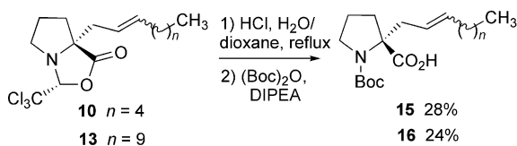
Scheme 4. Hydrolysis and N -protection of oxazolidinones 10 and 13 .
