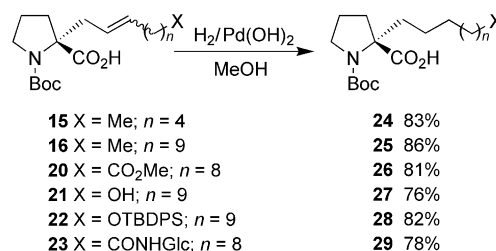
Scheme 6. Hydrogenations of alkenes 15 , 16 , 20–23 .
