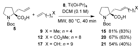
Scheme 5. CM between 5 and olefins 9 , 12 , and 17 (2 equiv.) in the presence of catalyst 8 (5 mol-%) and Ti(O i Pr) 4 (20 mol-%). In parentheses are yields of products under the same conditions in the absence of Ti(O i Pr) 4 .
