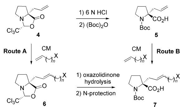
Scheme 2. Two complementary synthetic routes for prolines 7 .
