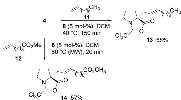
Scheme 3. CM of allylproline 4 with alkenes 11 and 12 .
