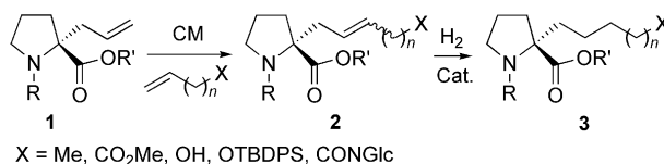
Scheme 1. General approach to \alpha -substituted prolines.
